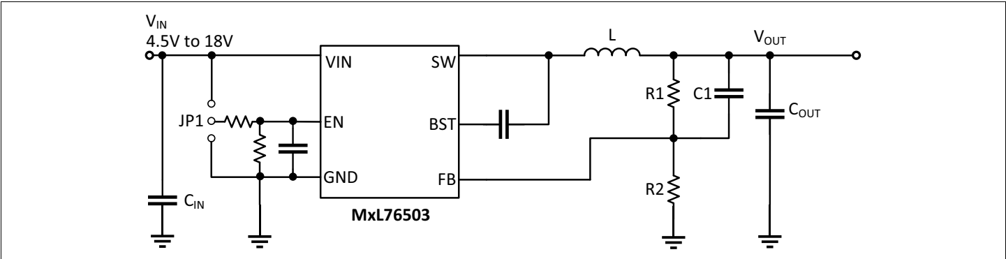
Figure 2: MxL76503 EVK Simplified Block Diagram
