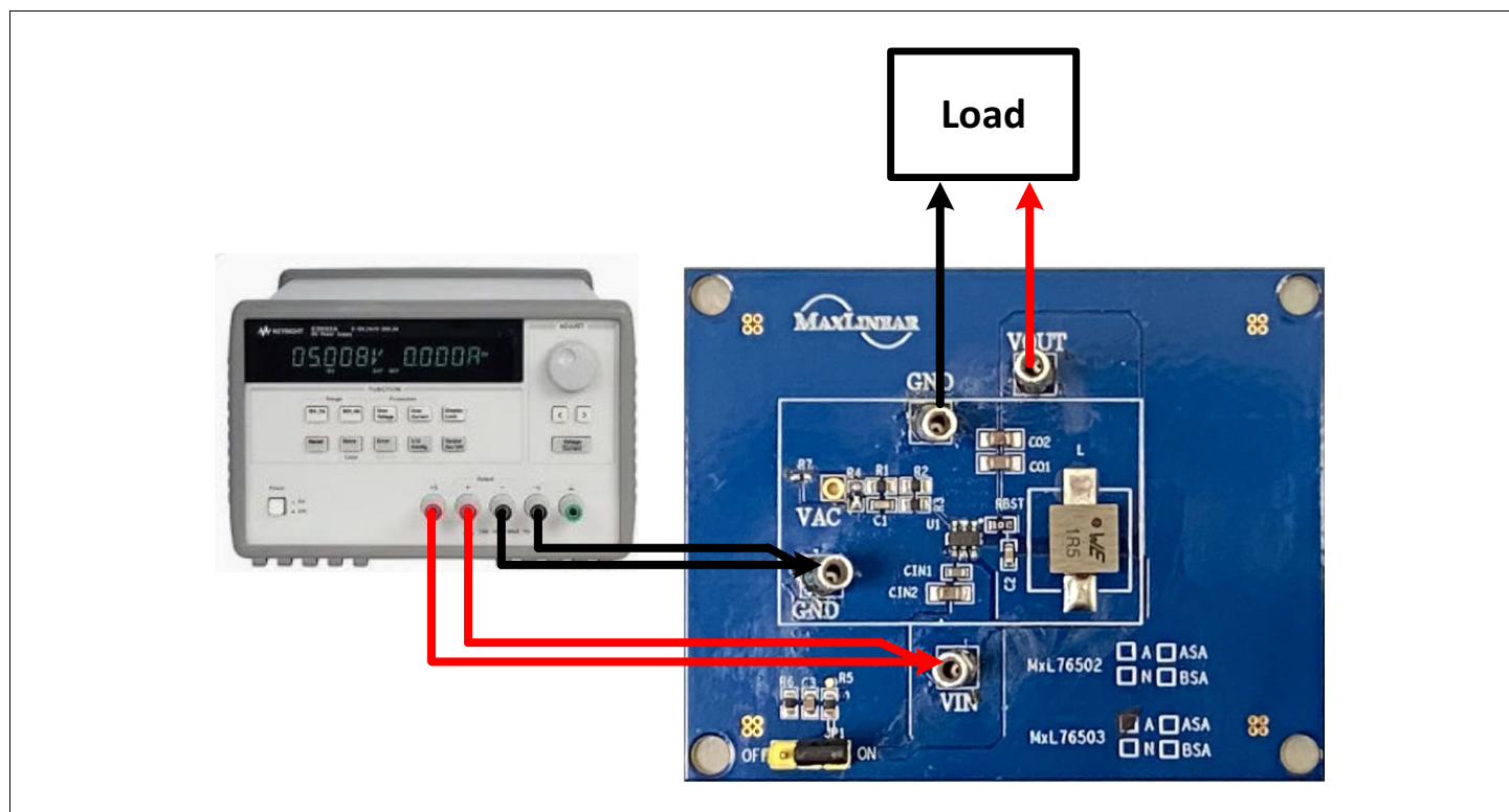
Figure 3: V_{IN} and V_{OUT} Connections of the MxL76503 EVK
