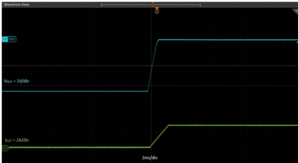
Figure 4: MxL76503 Start-Up with a 3A Load
