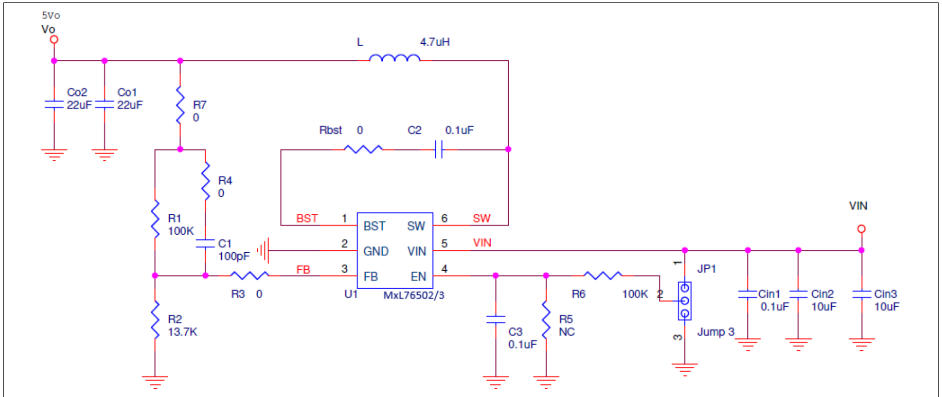
Figure 6: EVK Schematic
