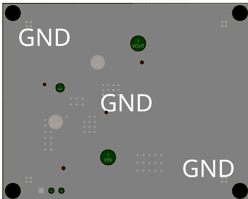
Figure 11: EVK PCB Layer 2
