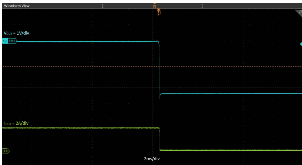
Figure 5: MxL76503 Shutdown with a 3A Load
